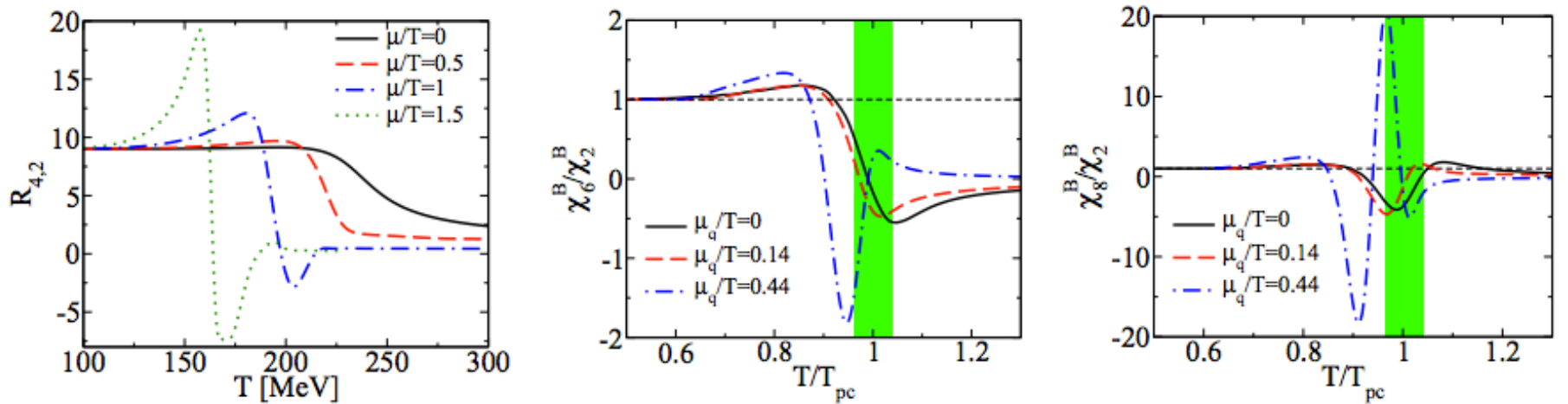
Figure 1. The temperature dependence of kurtosis R_{4,2} := 9\chi_4^B / \chi_2^B and the higher order, \chi_6^B / \chi_2^B and \chi_8^B / \chi_2^B , ratios of cumulants for different \mu_q/T calculated in the PQM model within the FRG approach [6, 8]. The T_{pc} is the pseudo-critical temperature obtained in the model at the physical pion mass.
