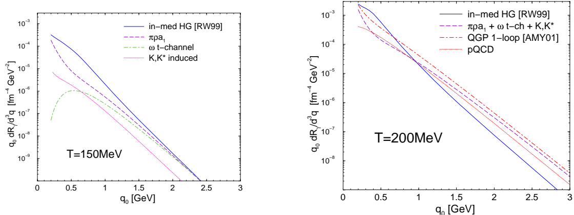
Figure 15: Thermal photon production rates in hot hadronic matter [108] (left panel), and compared to 1-loop [109] and full leading-order [110] QGP emission (right panel).
