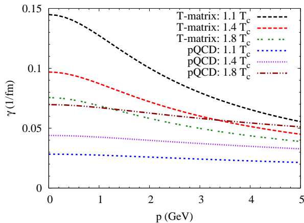
FIG. 3: Friction coefficients of charm quarks vs. 3-momentum for different temperatures in a QGP, based on our nonperturbative T -matrix approach (upper curves at p=0 ) and on LO pQCD scattering with \alpha_s=0.4 (lower curves).
