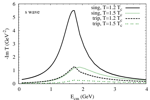
FIG. 1: Imaginary part of the in-medium T -matrix for S -wave c\bar{q} and cq scattering in color-singlet and antitriplet channels, respectively, at two different temperatures. The two-body threshold is at E_{\text{thr}}=m_c+m_q=1.75 GeV.
