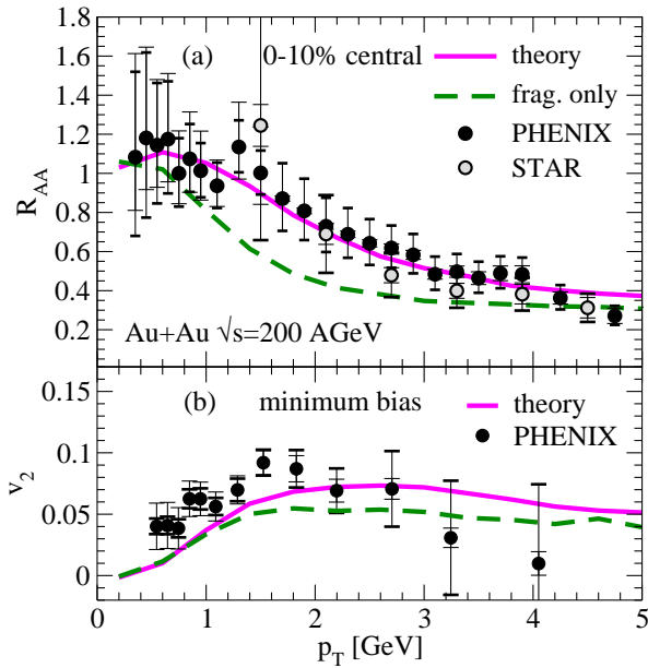
FIG. 4: Our results for the nuclear modification factor (upper panel) and elliptic flow (lower panel) of single electrons with/without (solid/dashed lines) quark coalescence in Au-Au collisions compared to RHIC data [5, 6]. The estimated theoretical uncertainty due to different extractions of the lQCD based heavy-light quark potentials is up to \sim 30\% [29].
