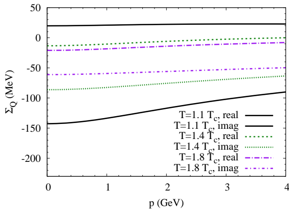
FIG. 2: Real (upper lines) and imaginary (lower lines) parts of the on-shell c -quark selfenergy versus 3-momentum at temperatures T=1.1, 1.4 and 1.8 T_c .
