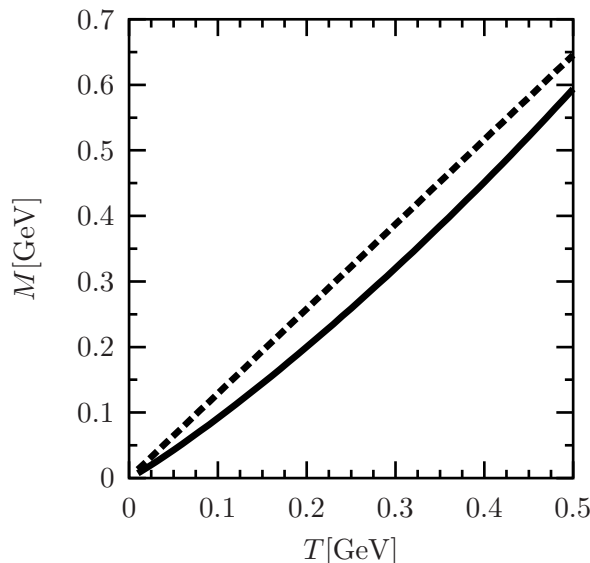
Figure 3.12: The numerical solution for (3.237). Both the perturbative (dashed line) and the self-consistent (solid line) are shown. As parameters \Lambda = 100\text{MeV} and \lambda = 40 were chosen.
