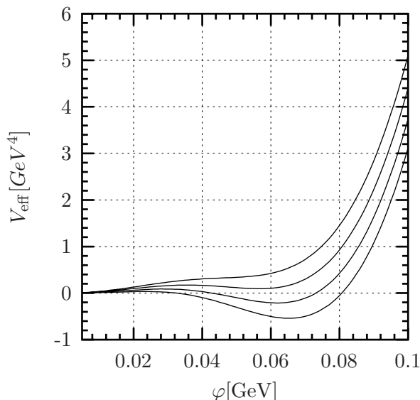
Figure 3.13: The evolution of the effective potential with temperatures between 150MeV and 180MeV. The potential is fixed to V_{\text{eff}}(\varphi = 0) = 0 for all temperatures.
