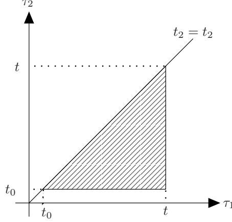
Figure 2.1: Range of integration variables in (2.21)
