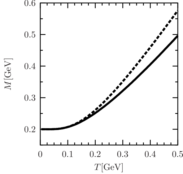
Figure 3.11: The numerical solution for (3.236). Both the perturbative (dashed line) and the self-consistent (solid line) are shown. As parameters m = 200\text{MeV} and \lambda = 40 were chosen.
