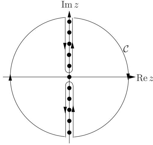
Figure A.2: Integration path in (A.12).
